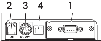
RS: Serial RS-232C + USB
