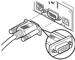
Serial interface
