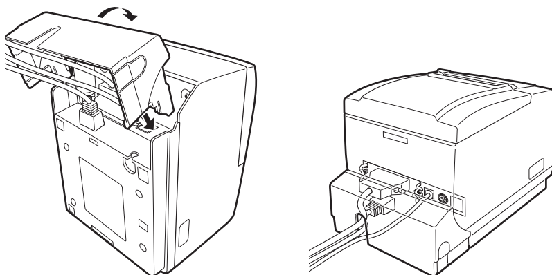
CT-S6011IS
