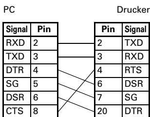
9-Pin – 25-Pin-Kabel
